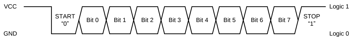
Figure 28. UART 8 – 1 Signaling
