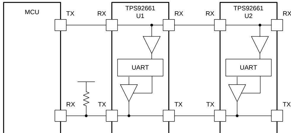
Figure 27. Communications Connections
